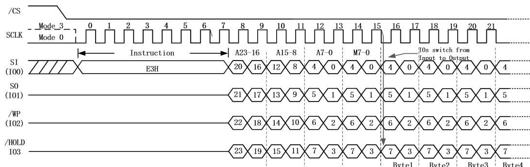
Figure 17.a. Octal Word Read Quad I/O Instruction (Initial instruction or previous M5-4 \neq 10, SPI Mode only)
