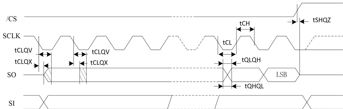
Figure 47. Output Timing
