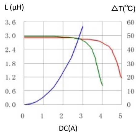
6. CD43T125NP-3R3MC
