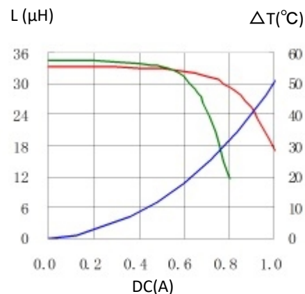
18. CD43T125NP-330KC
