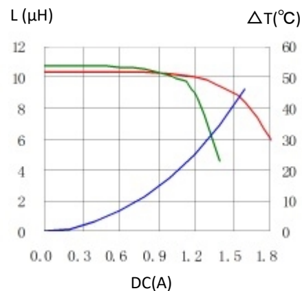
12. CD43T125NP-100MC
