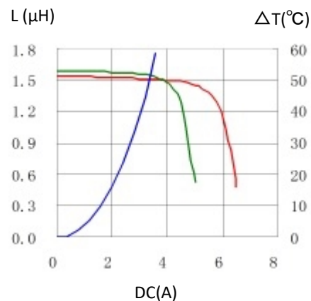
3. CD43T125NP-1R8MC
