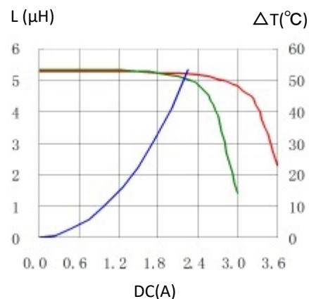
9. CD43T125NP-5R6MC
