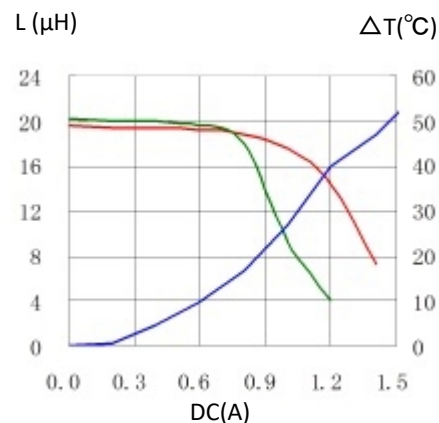
15. CD43T125NP-180MC
