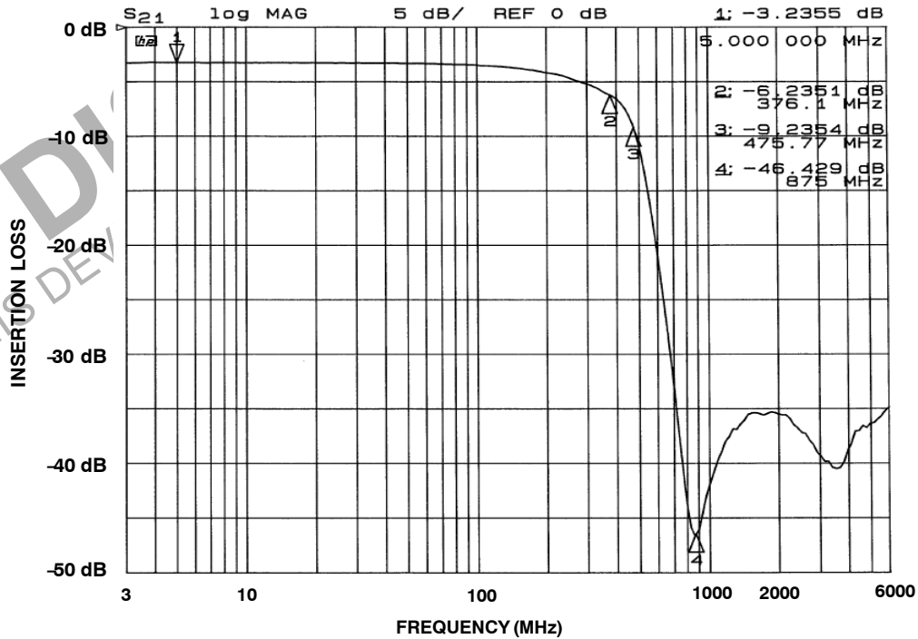
Figure 2. Insertion Loss vs. Frequency (2.5 V Bias)
