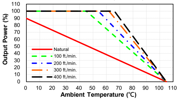
CQB150-300S05 Derating Curve with Heatsink QBT210 (Vin=300V)
