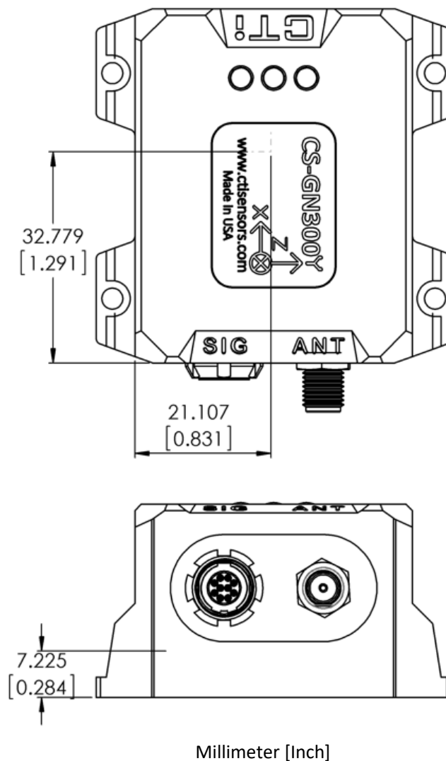
Figure 1. Location of the IMU Center of Measurement
