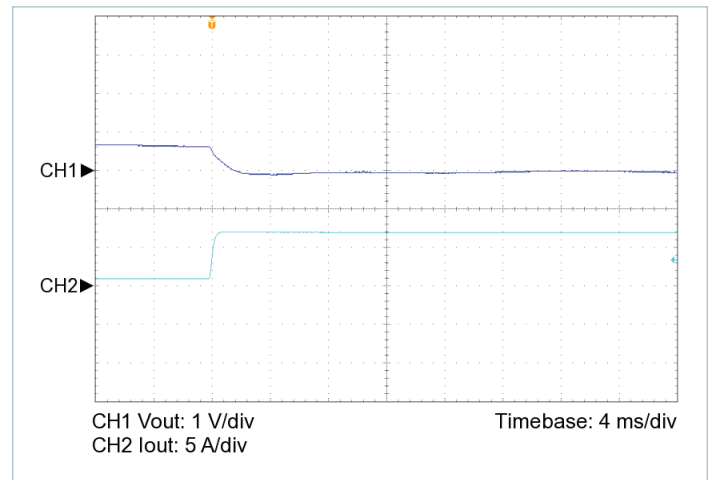
Figure 23 — 10 – 100% load transient response, V_{IN} = 43\text{V} , nominal trim, C_{OUT\_EXT} = 1000\mu\text{F}
