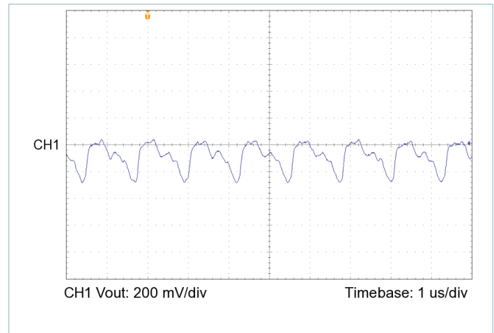
Figure 18 — Output voltage ripple, V_{IN} = 43\text{V} , V_{OUT} = 15.0\text{V} , C_{OUT\_EXT} = 1000\mu\text{F} , R_{LOAD} = 2.239\Omega
