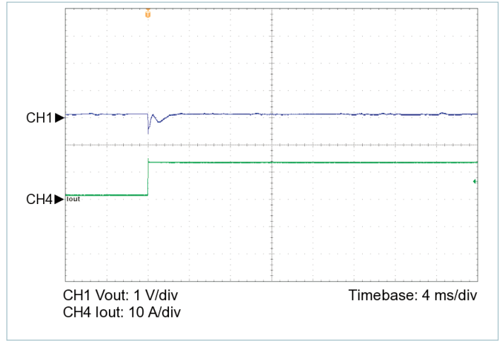
Figure 6 — 10% to 100% load transient response, V_{IN} = 48\text{ V} , nominal trim, C_{OUT\_EXT} = 1000\ \mu\text{F}
