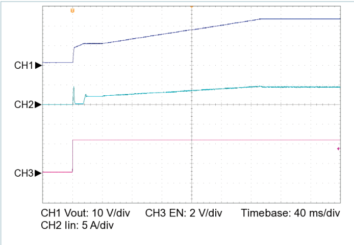
Figure 15 — Startup from EN, V_{IN} = 48\text{ V} , C_{OUT\_EXT} = 10000\ \mu\text{F} , R_{LOAD} = 1.800\ \Omega
