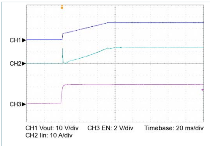
Figure 20 — Start up from EN, V_{IN} = 24\text{V} , C_{OUT\_EXT} = 6800\mu\text{F} , R_{LOAD} = 0.701\Omega
