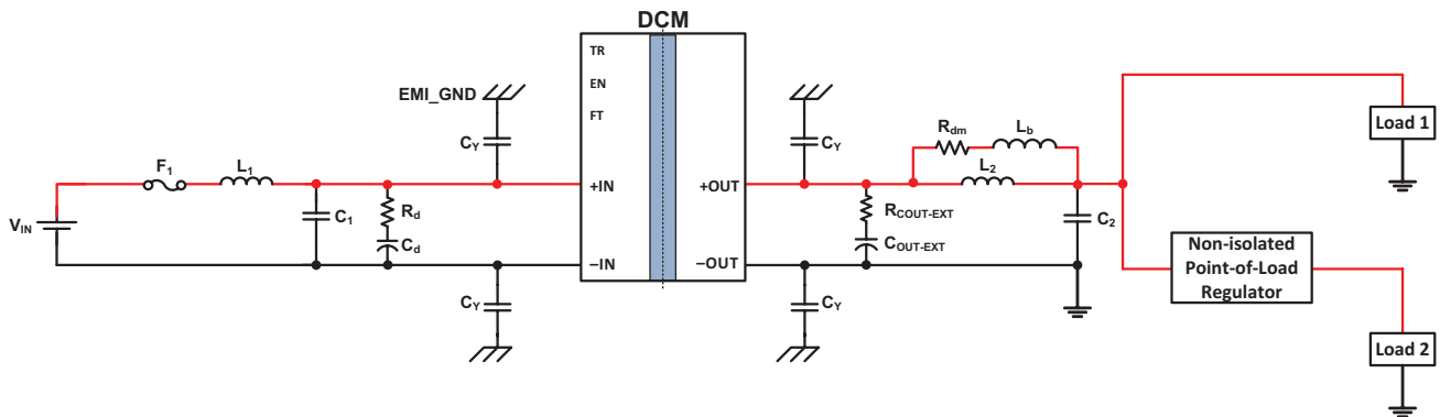
Typical application 2: single DCM3623x36G17C2yzz, to a non-isolated regulator, and direct to load
