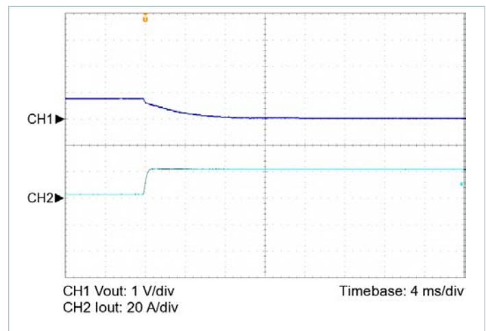
Figure 8 — 10 – 100% load transient response, V_{IN} = 24\text{V} , nominal trim, C_{OUT\_EXT} = 680\mu\text{F}
