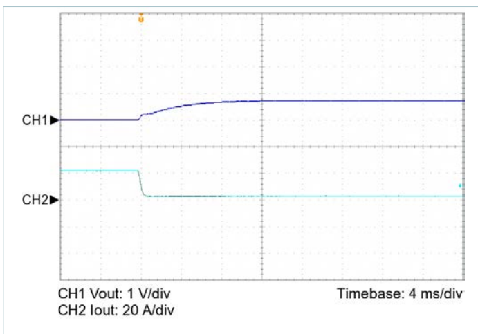
Figure 7 — 100 – 10% load transient response, V_{IN} = 24\text{V} , nominal trim, C_{OUT\_EXT} = 680\mu\text{F}
