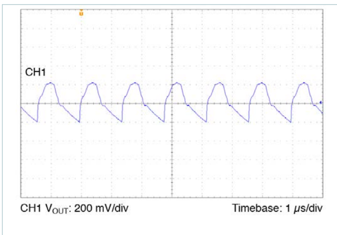
Figure 22 — Output voltage ripple, V_{IN} = 24\text{V} , V_{OUT} = 15.0\text{V} , C_{OUT\_EXT} = 680\mu\text{F} , R_{LOAD} = 0.701\Omega
