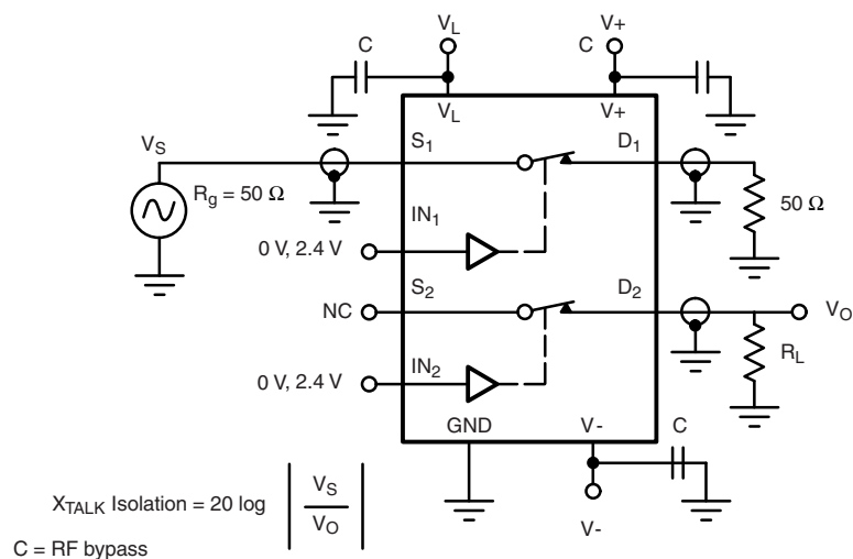
Fig. 5 - Crosstalk
