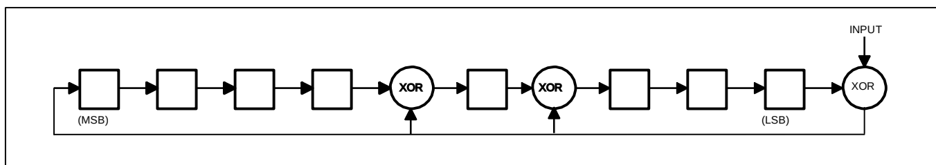
Figure 9. CRC Generator
