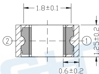
Recommend Soldering Pad
