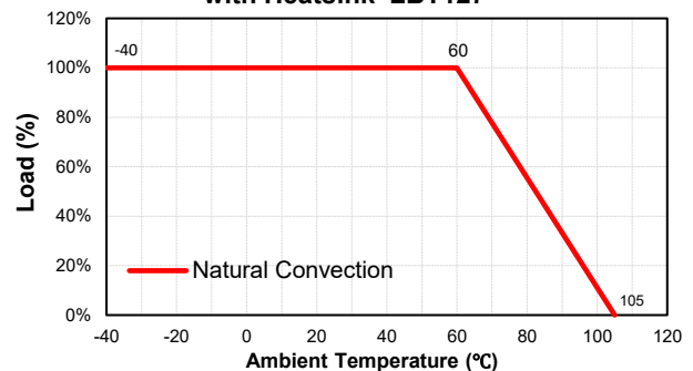
ECLB60W Derating Curve with Heatsink LBT127
