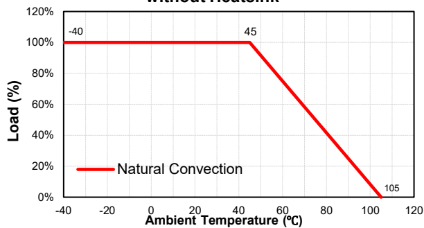
ECLB60W Derating Curve without Heatsink
