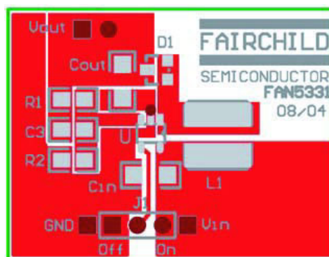
Figure 14. Recommended Layout
