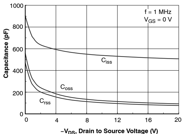
Figure 19. Capacitance Characteristics
