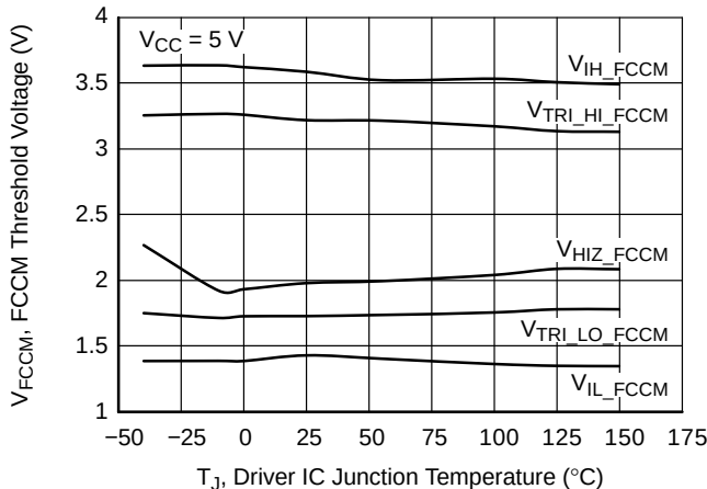
Figure 20. FCCM Threshold vs. Temperature
