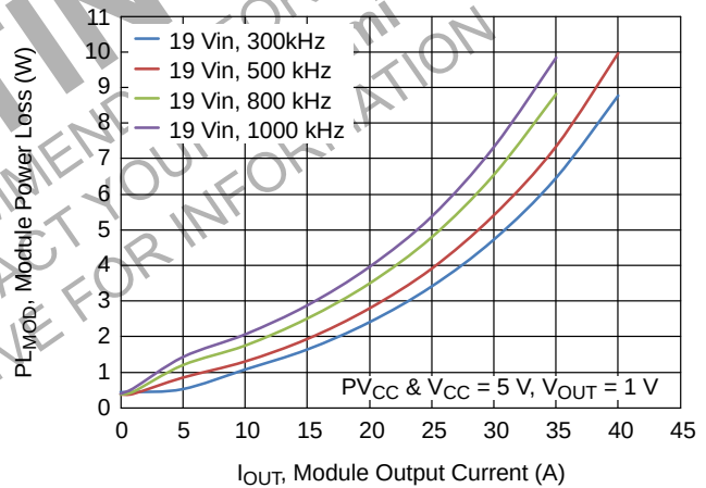
Figure 7. Power Loss vs. Output Current with 19 V_{IN}
