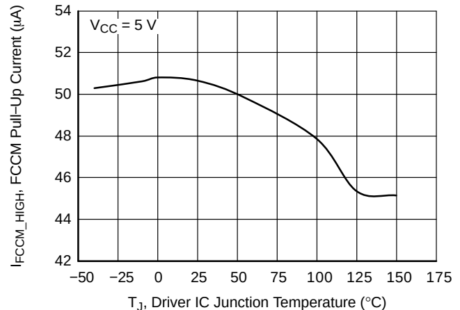
Figure 21. FCCM Pull-Up Current vs. Temperature
