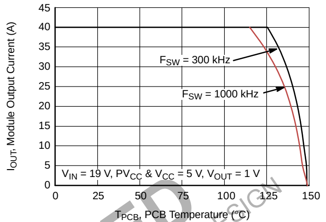
Figure 5. Safe Operating Area with 19 V_{IN}
