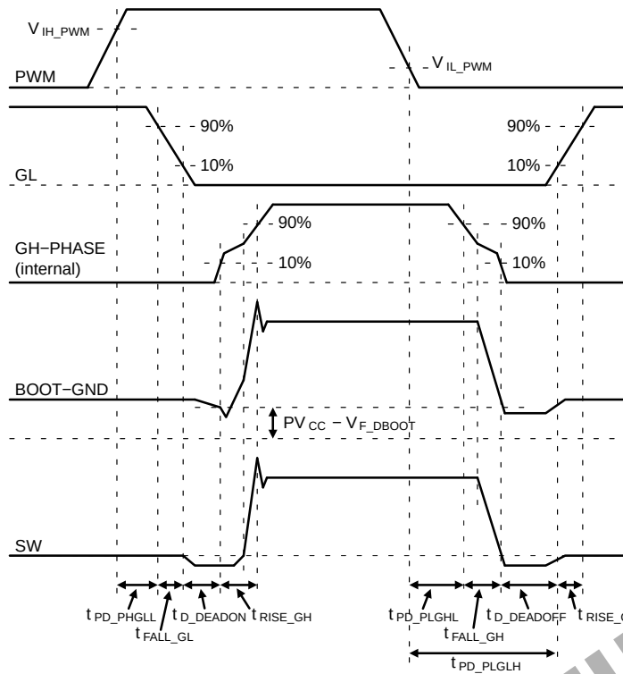
Figure 25. PWM Timing Diagram
