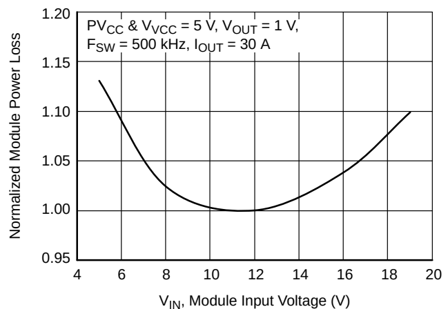
Figure 9. Power Loss vs. Input Voltage
