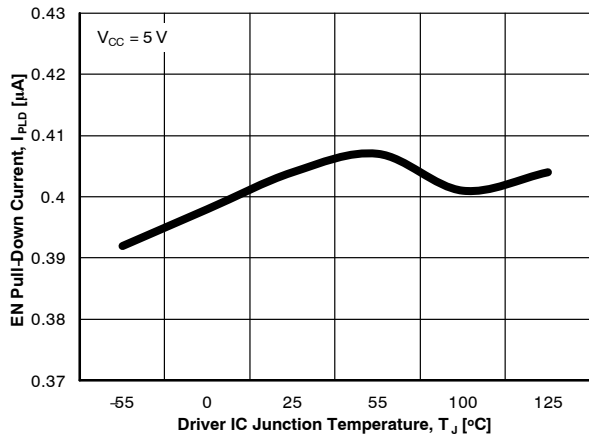
Figure 24. EN Pull-Down Current vs. Temperature
