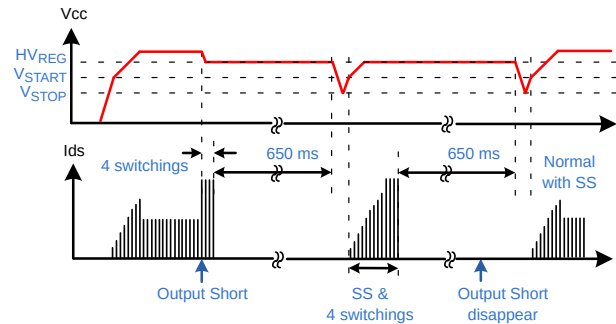
Figure 24. AOCPS Waveform
