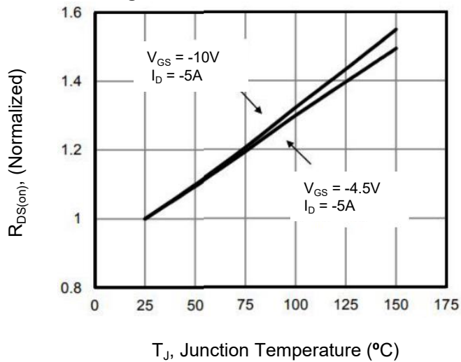
Figure 7. Drain-Source On-Resistance
