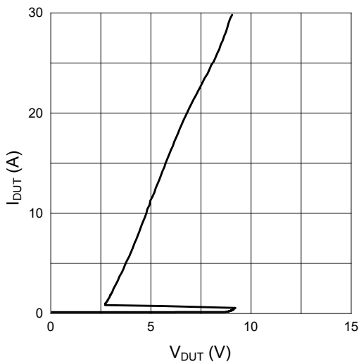
Figure 5. Transmission Line Pulse ( T_p=100\text{ns} )
