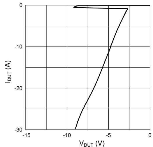
Figure 6. Transmission Line Pulse ( T_p=100\text{ns} )
