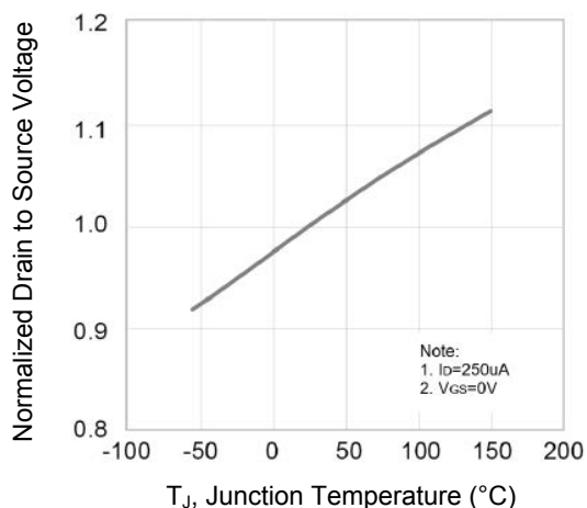
Figure 5. Normalized BV_{DSS} vs. Junction Temperature
