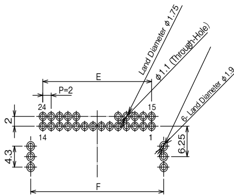
Connector Side Recommended PCB Dimensions and Pin No.
