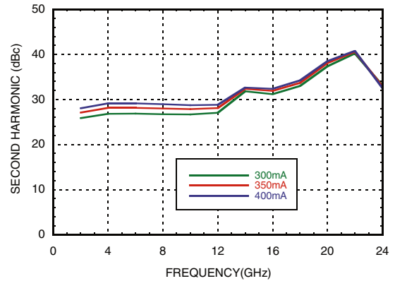
Second Harmonics vs. Idd @ Pout = + 18dBm
