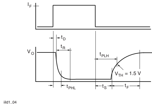
Fig. 6 - Saturated Switching Timing
