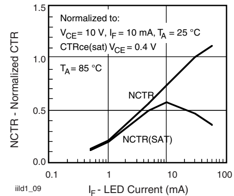
Fig. 11 - Normalized Non-Saturated and Saturated CTR vs. LED Current
