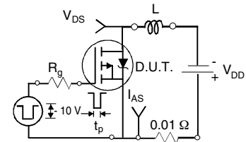
Fig. 10a - Switching Time Test Circuit
