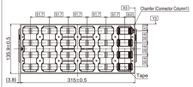
JEDEC Tray for IT3D 200 Position Receptacles
