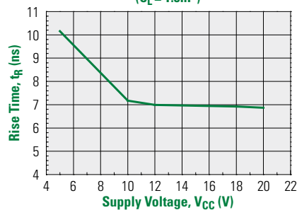
Rise Time vs. Supply Voltage ( C_L = 1.8\text{nF} )
