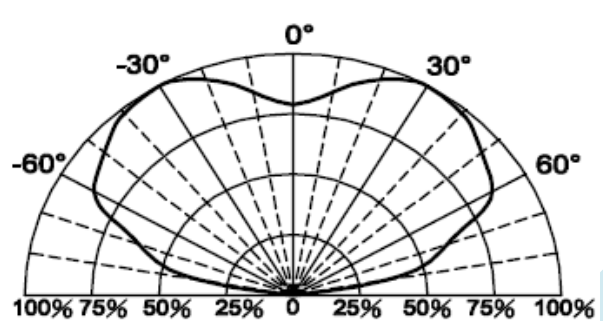
Fig.6 Directive Radiation
