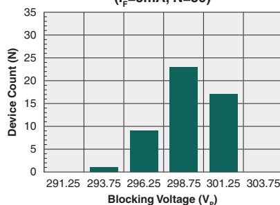
Typical Blocking Voltage Distribution ( I_F=5\text{mA} , N=50)
