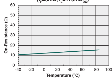
Typical On-Resistance vs. Temperature ( I_F=0\text{mA} , I_L=170\text{mA}_{DC} )
