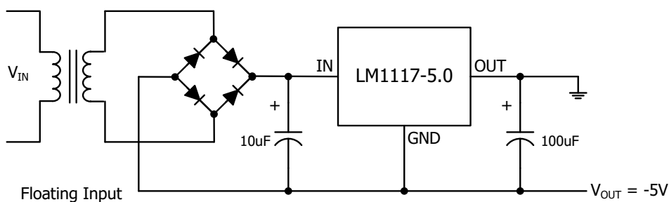
Fig.3 Negative Supply
