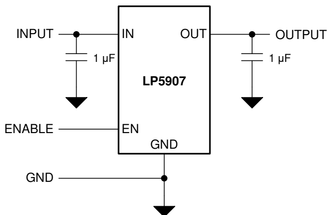
Figure 7-1. LP5907 Typical Application
