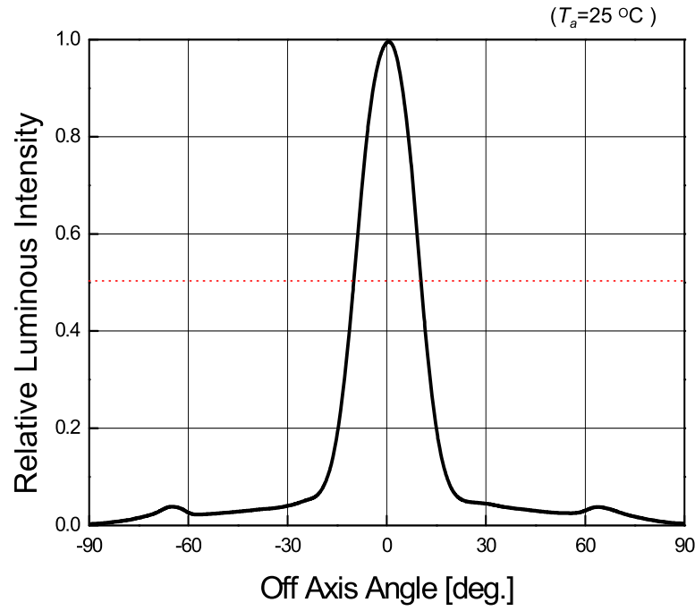
Radiation Diagram
