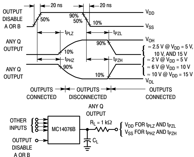
Figure 2. Three-State Propagation Delay Waveshape and Circuit
