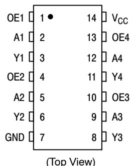
Figure 2. Pinout: 14-Lead Packages
