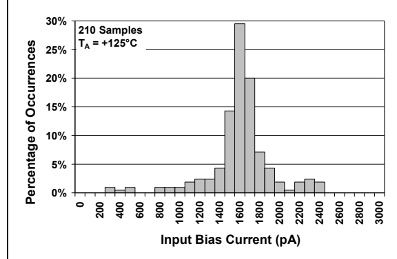
FIGURE 2-5: Input Bias Current at T_A = +125^\circ\text{C} .
