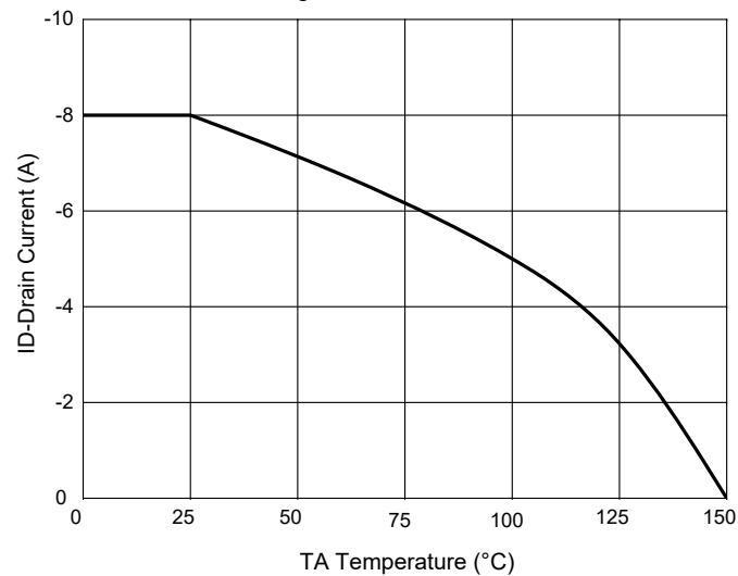
Fig. 10 - Drain Current
