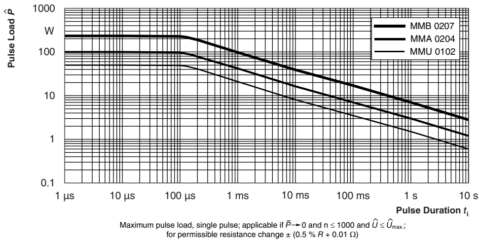
Single Pulse for R \geq 10 \Omega
