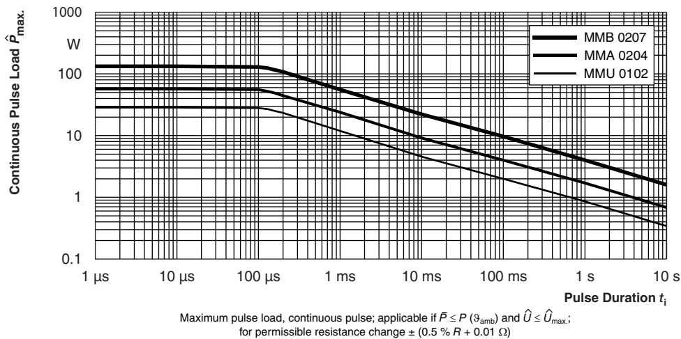
Continuous Pulse for R \geq 10 \Omega
