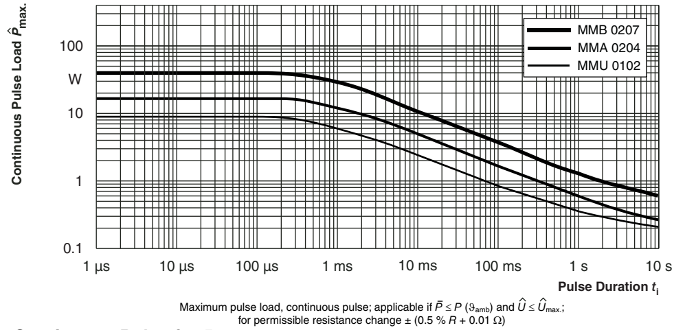
Continuous Pulse for R < 10 \Omega
