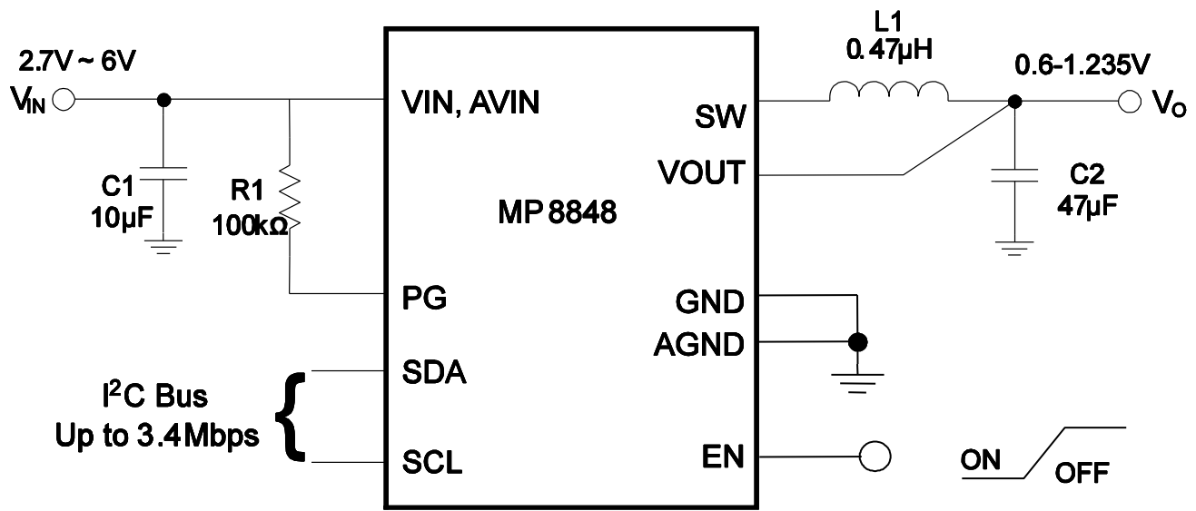
Figure 3: Application Circuit
