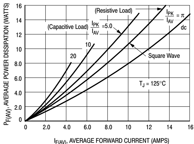
Figure 10. Power Dissipation
