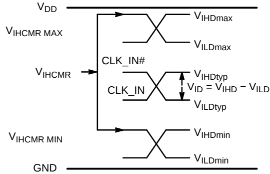
Figure 8. V_{IHCMR} Diagram
