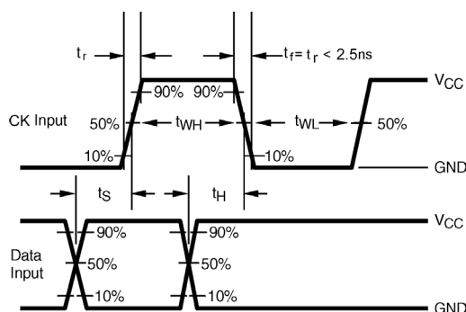
Figure 5. AC Waveforms
