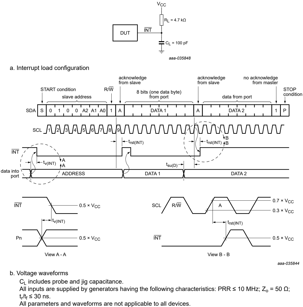
Fig. 26. Interrupt load circuit and voltage waveforms
