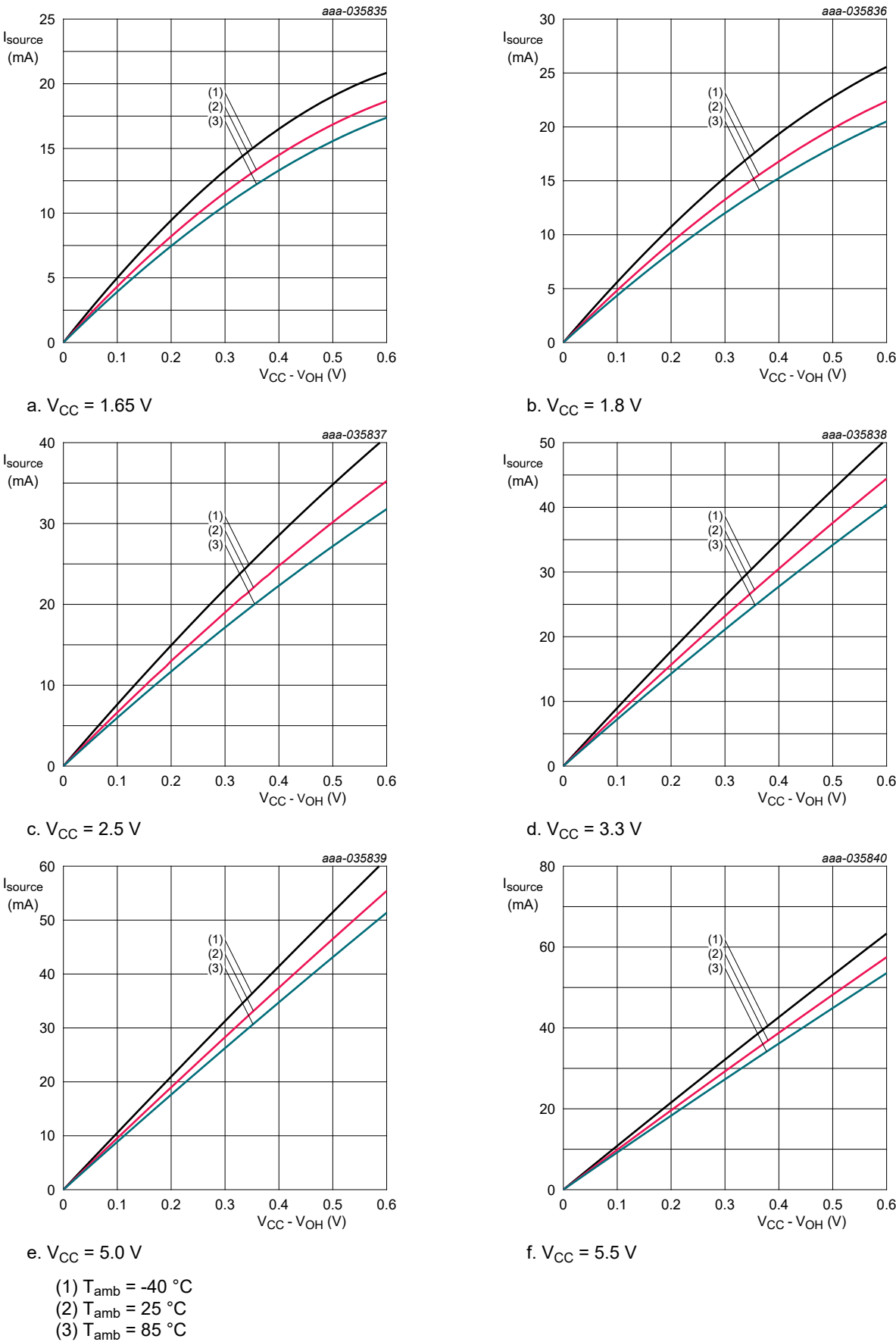
Fig. 22. I/O source current versus HIGH-level output voltage
