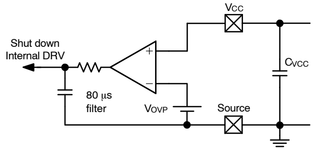
Figure 46. Realization of OVP Protection on VCC Pin
