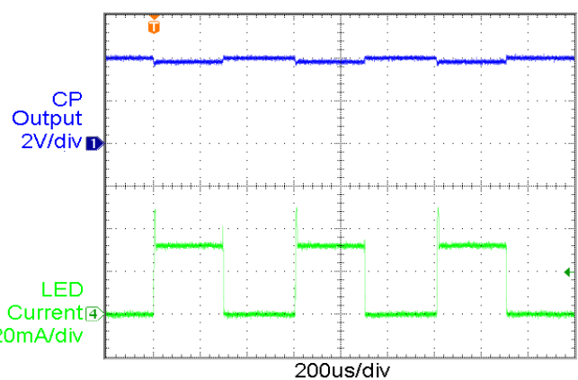
Figure 9. Power Up in 1.33x Mode, I_{LED} = 30\text{ mA/ch}
