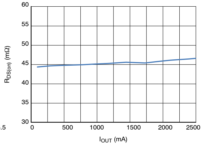
Figure 5. R_{DS(on)} (mΩ) vs. I_{load} (mA) at 3.6 V
