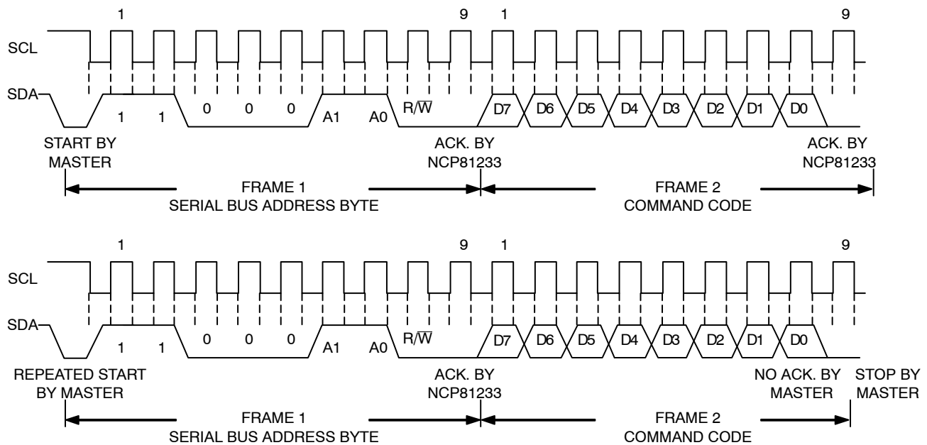
Figure 21. Read Byte
