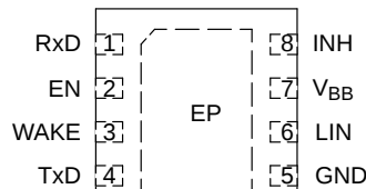
DFN8 (Top View)
