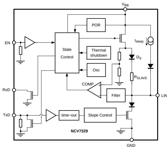
Figure 1. Block Diagram
