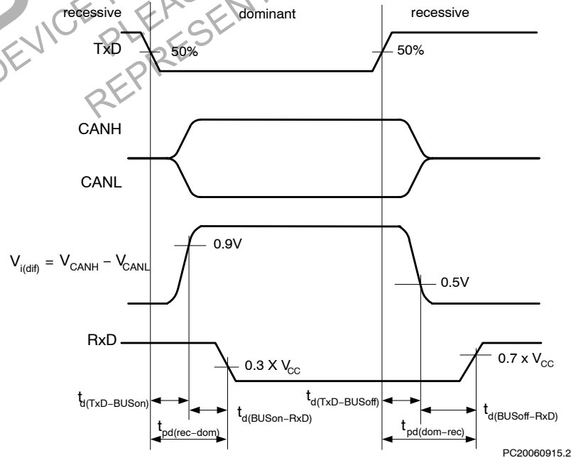
Figure 6. Timing Diagram for AC Characteristics
