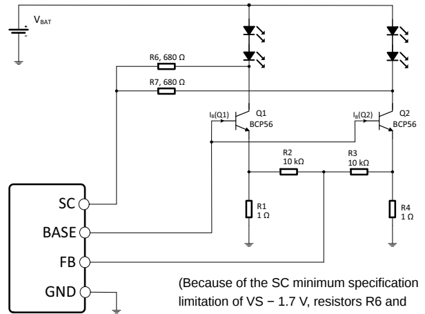
Figure 17. Driving Multiple Strings
